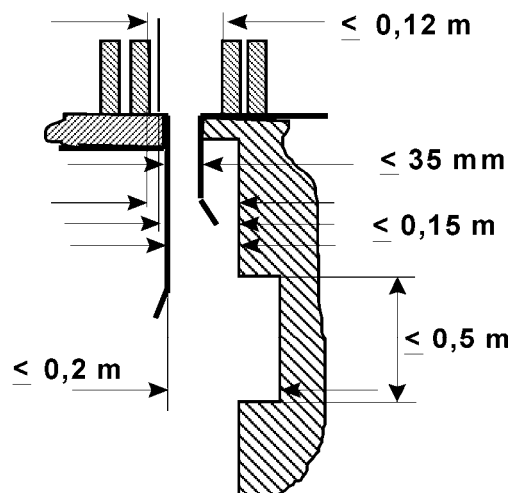
Figure 5 — Clearances between car and wall facing the car entrance
